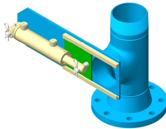
Unit with NPT and Flange
